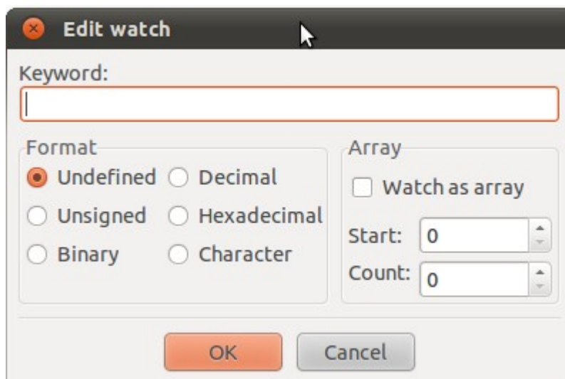
Figura 11: Add watch
