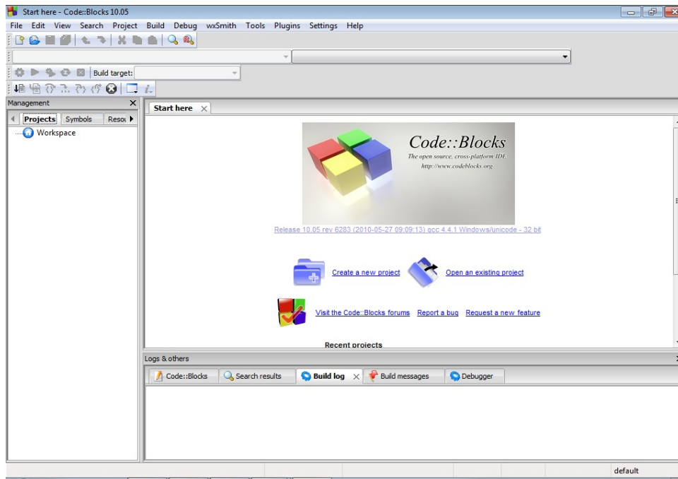
Figura 1: IDE Code::Blocks
