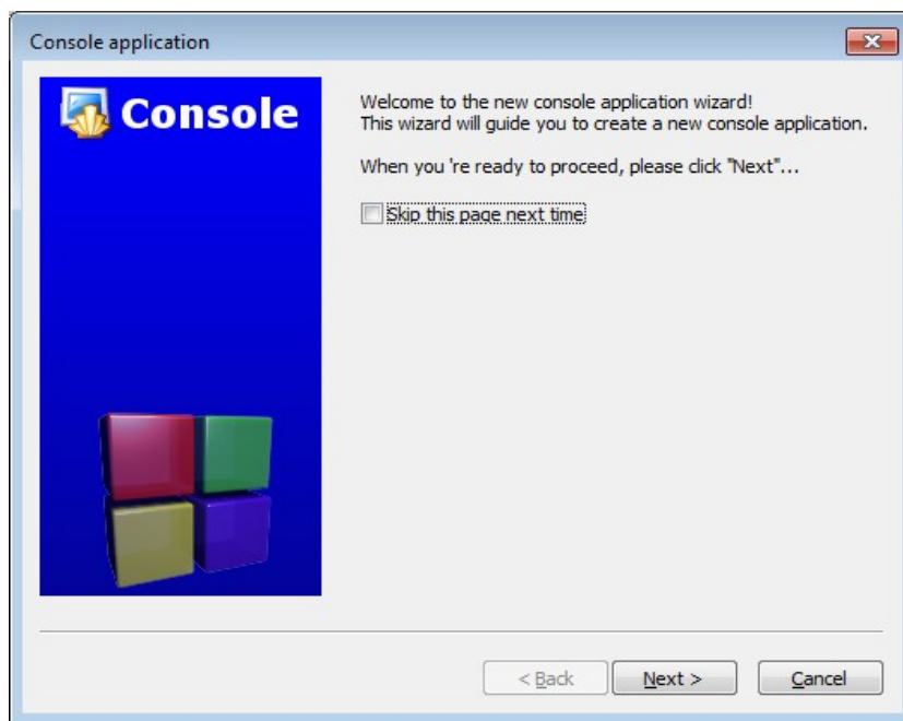
Figura 3: Console Application
